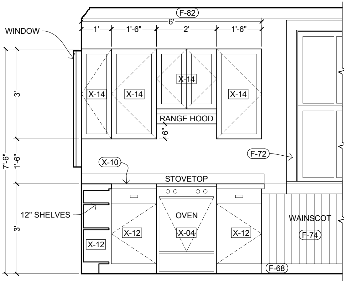
1 KITCHEN ELEVATION SCALE: 1/2" = 1'-0"
