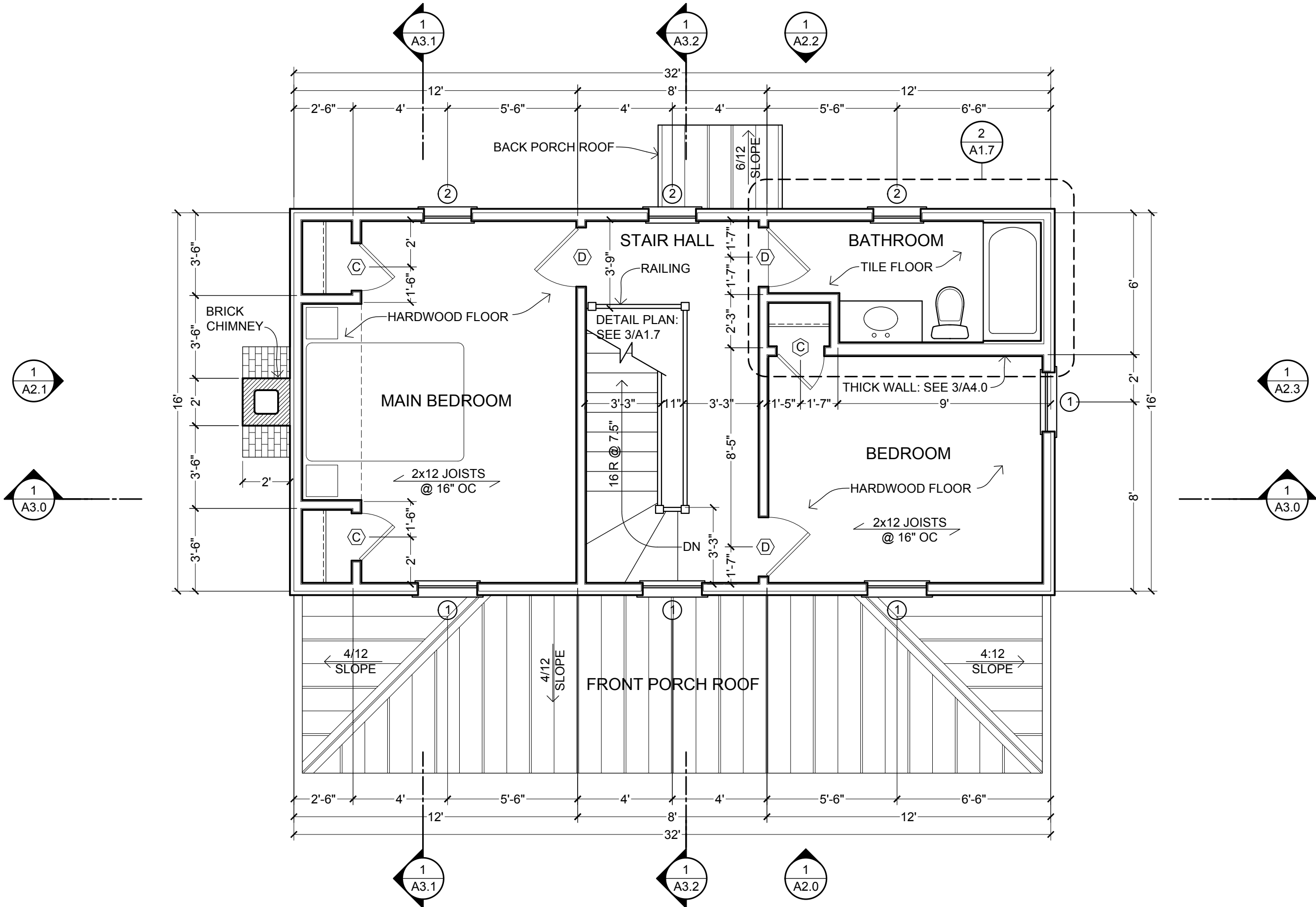
1 2ND FLOOR PLAN SCALE: 1/4" = 1'-0"
