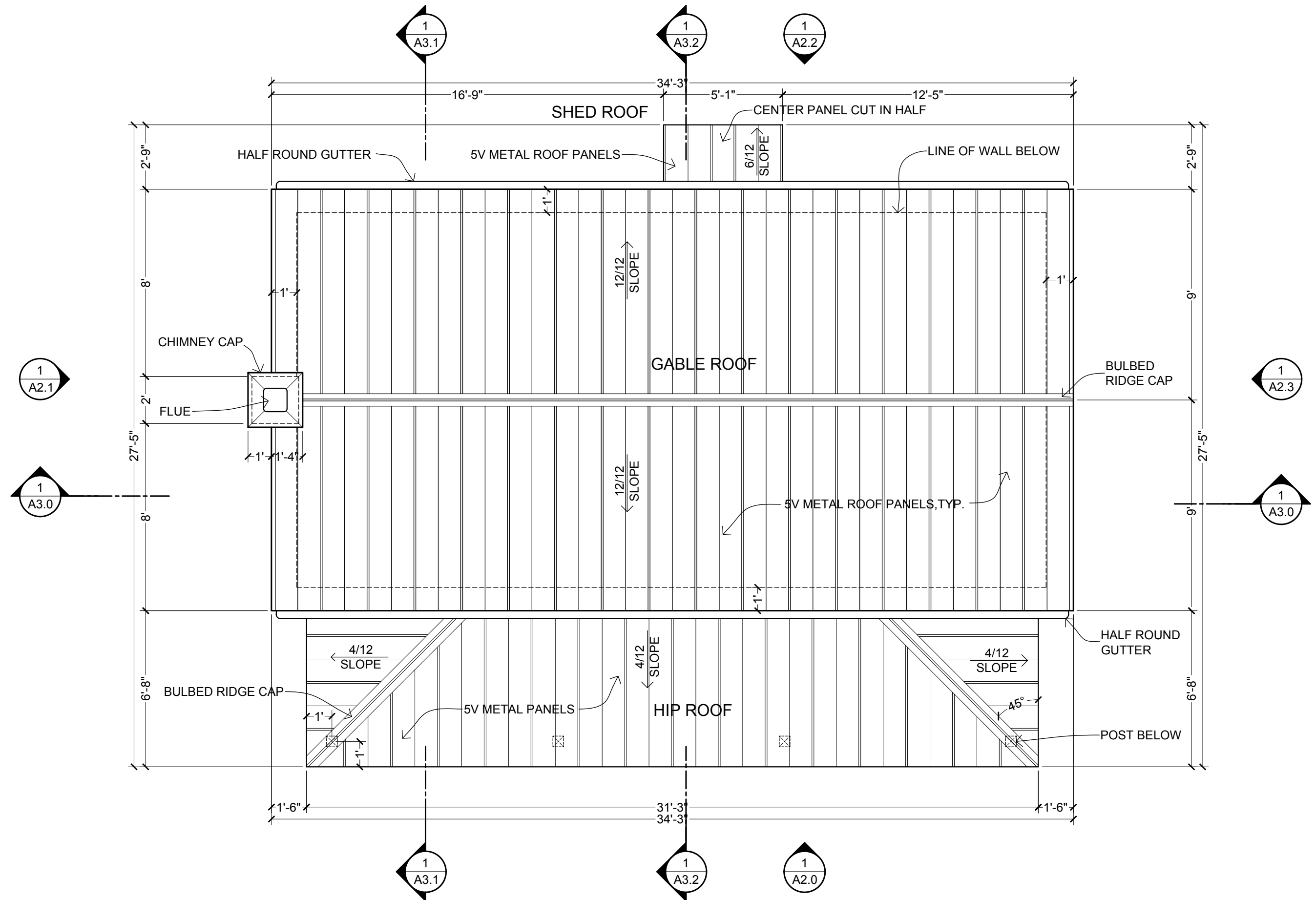
1 ROOF PLAN SCALE: 1/4" = 1'-0"
