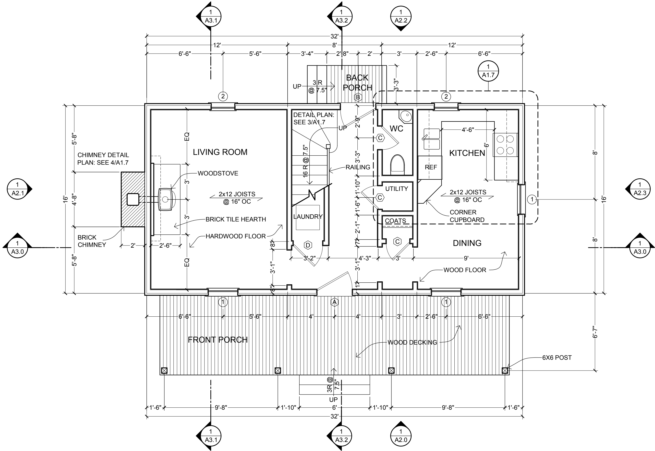
1 1ST FLOOR PLAN SCALE: 1/4" = 1'-0"
