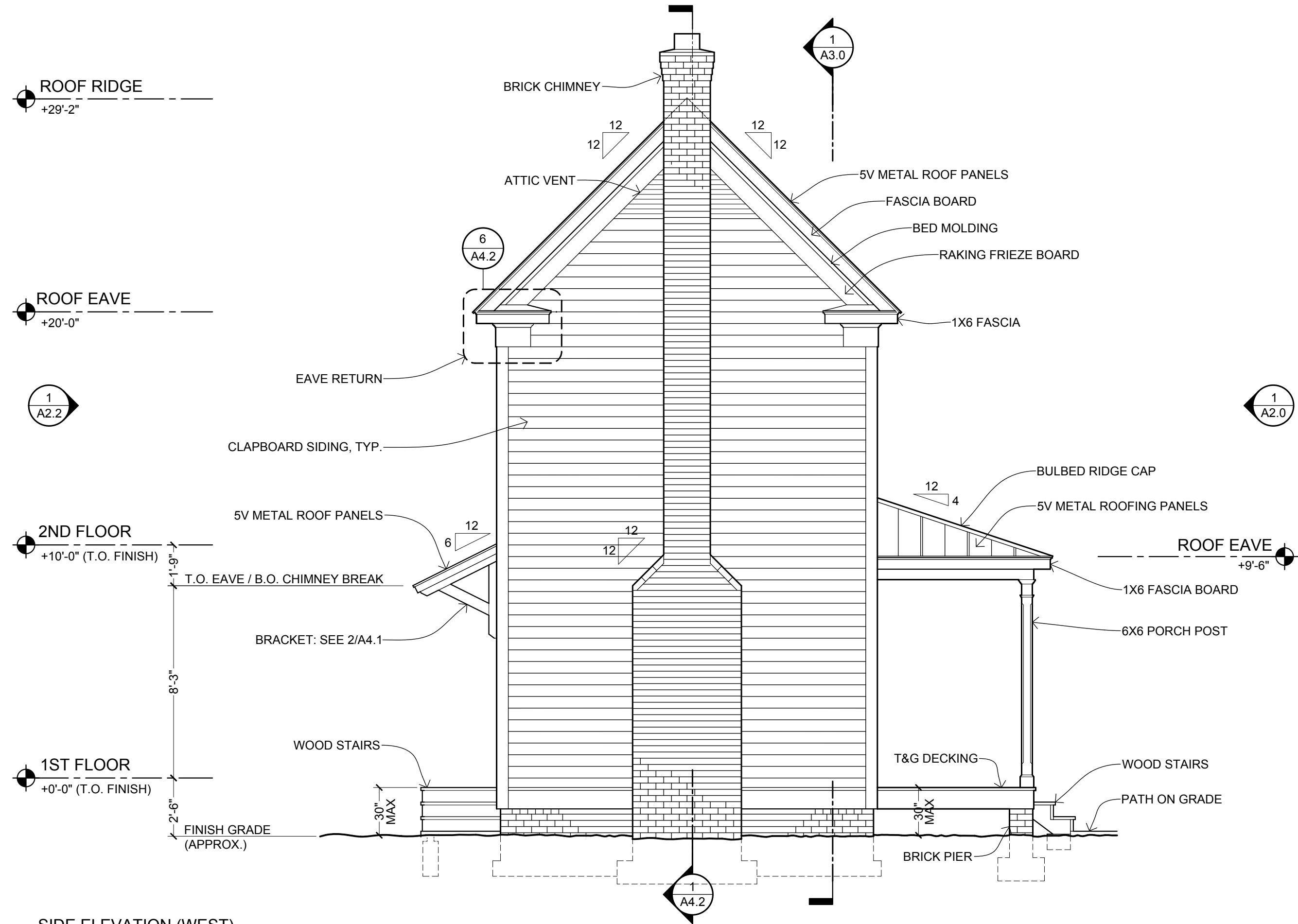
1 SIDE ELEVATION (WEST) SCALE: 1/4" = 1'-0"
